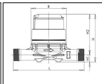
DN20 composite
