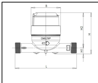
DN 20 brass
