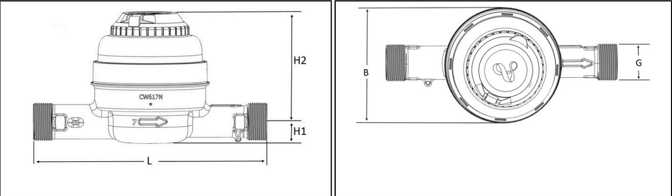
Front view - DN40
