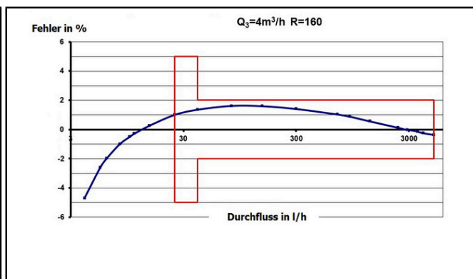
Q_3=4 R160
