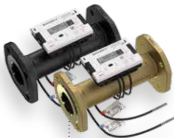
SHARKY 775: DN 65 Q_p 25 m 3 /h
