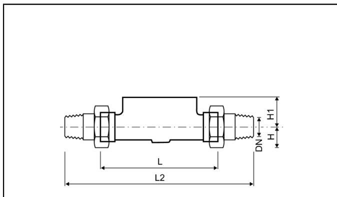
Housing
